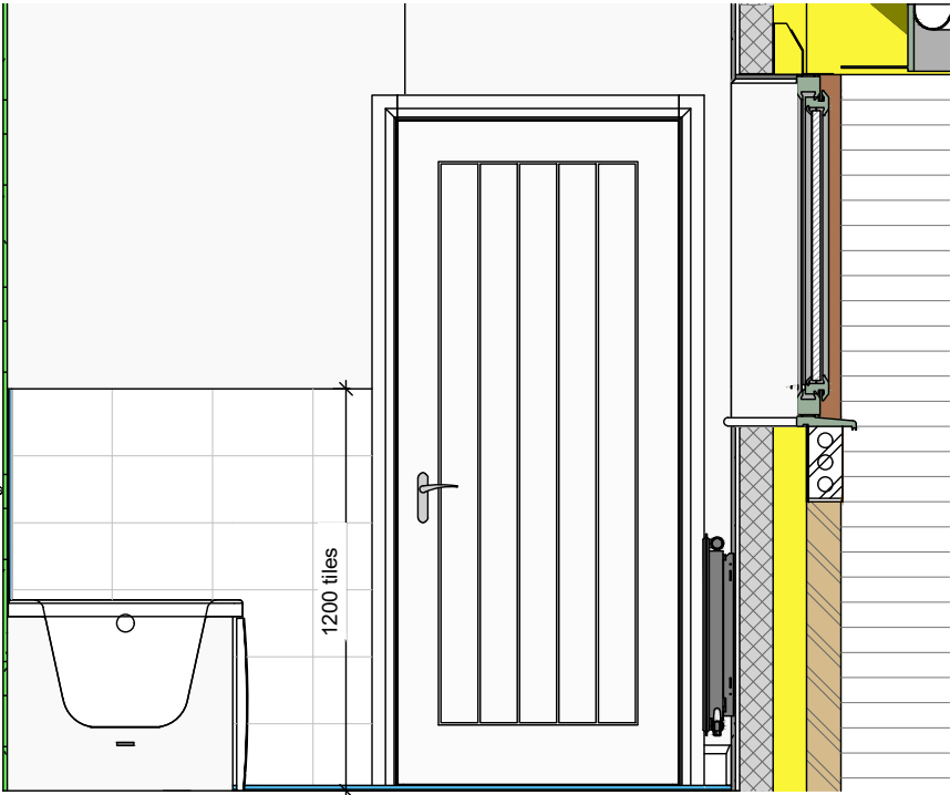
A Bathroom - View A 1 : 25
