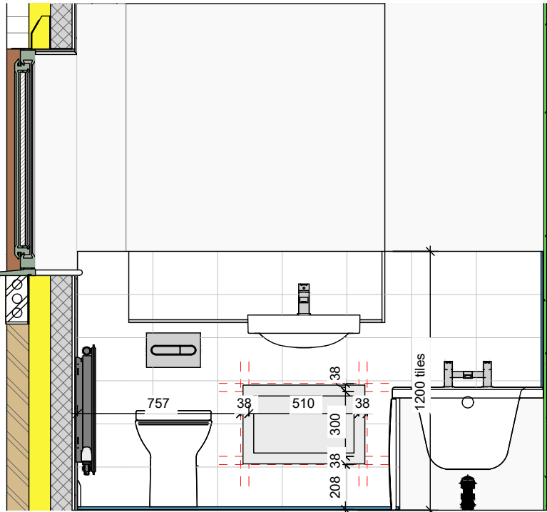
C Bathroom - View C 1 : 25
