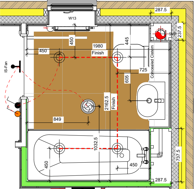
1 Bathroom Layout 1 : 25
